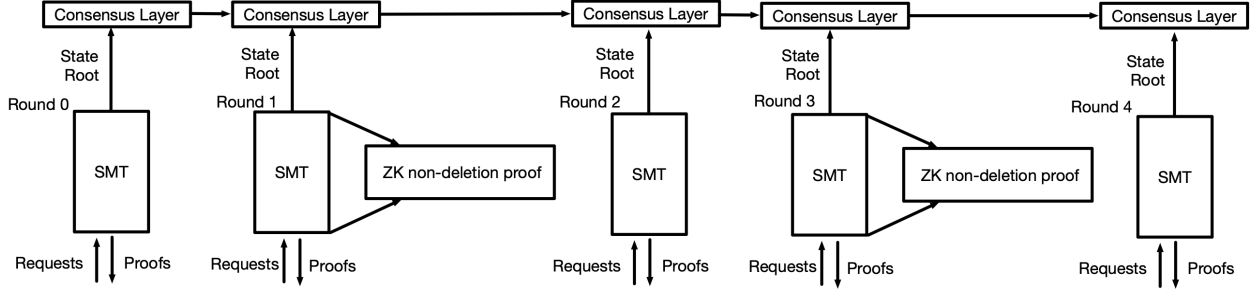
Figure 6: Proof Aggregation Layer
