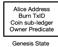
Figure 13: Agent Genesis State
