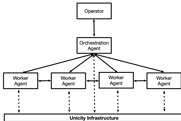
Figure 17: Agents coordinating on a task through trustless state verification
