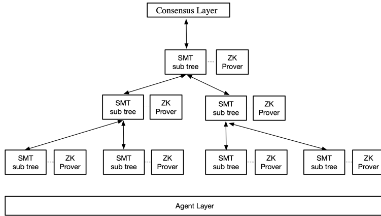
Figure 7: Aggregator Hierarchical Infrastructure
