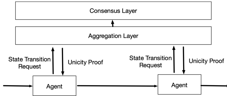
Figure 5: Agent to Agent Interaction
