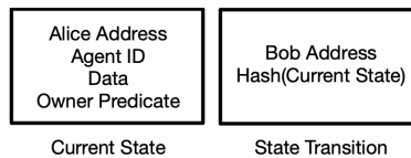
Figure 9: Current State and State Transition
