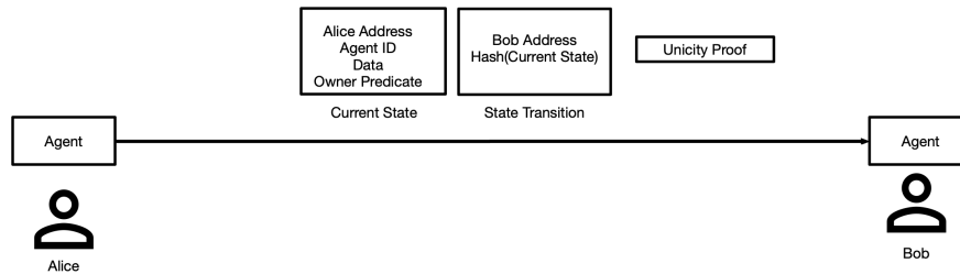
Figure 11: Agent Synchronization
