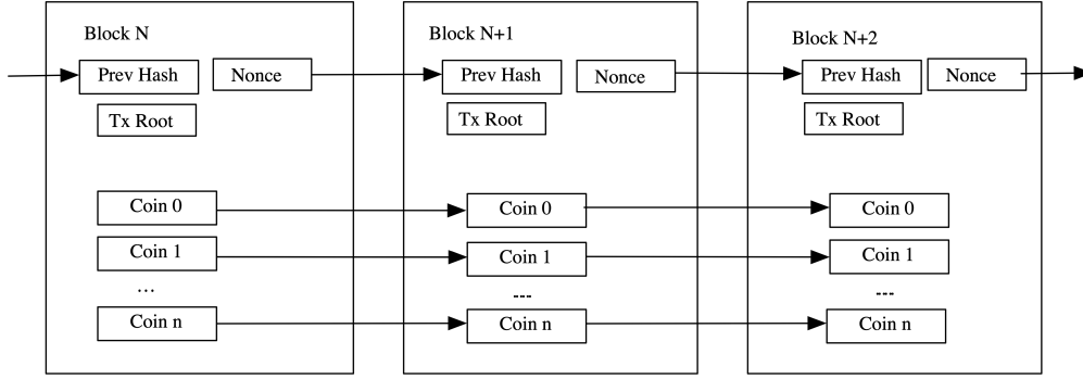
Figure 4: Decomposition into coin sub-ledgers
