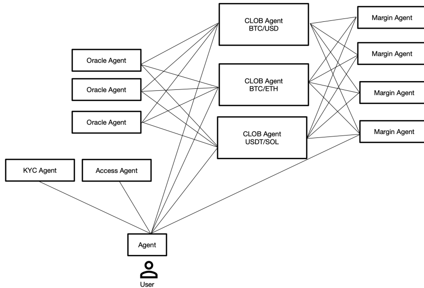
Figure 15: Agent-Based Decentralized Exchange
