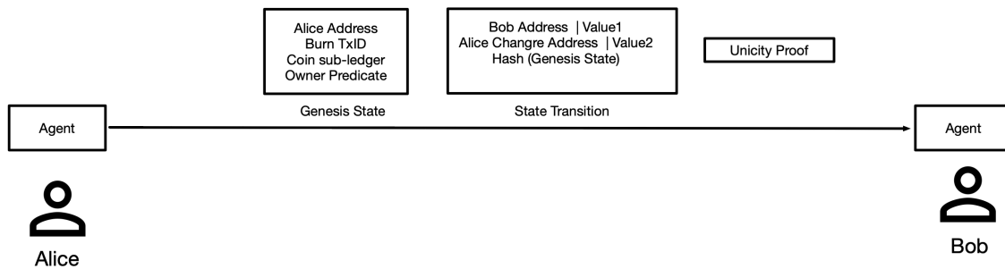
Figure 14: Transfer of a coin minted in the Contract Execution Layer
